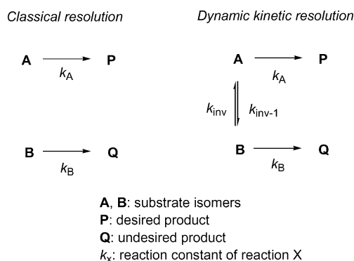
Figure 1. Comparison of classical resolution and dynamic kinetic resolution.
