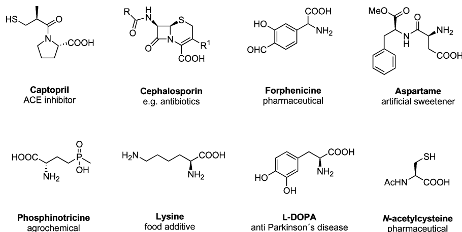
Scheme 1. Selection of industrially important \alpha -amino acids.
