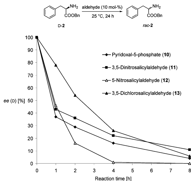
Figure 2. Comparison of enantioselectivity–time dependency of several salicylaldehydes and pyridoxal-5-phosphate ( 10 ).
