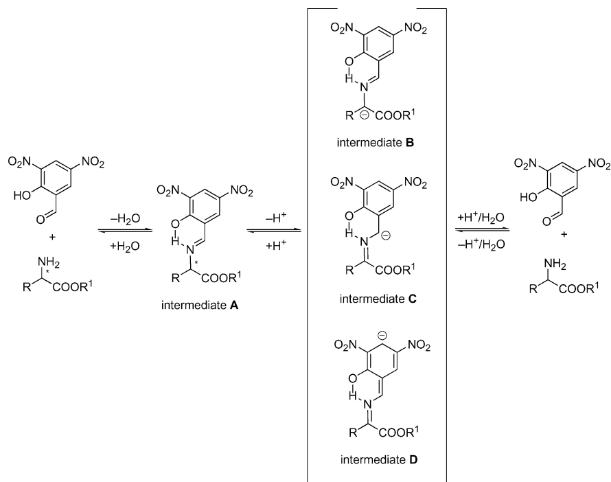
Scheme 2. Proposed mechanism for the aldehyde-catalyzed racemization of \alpha -amino acid esters.
